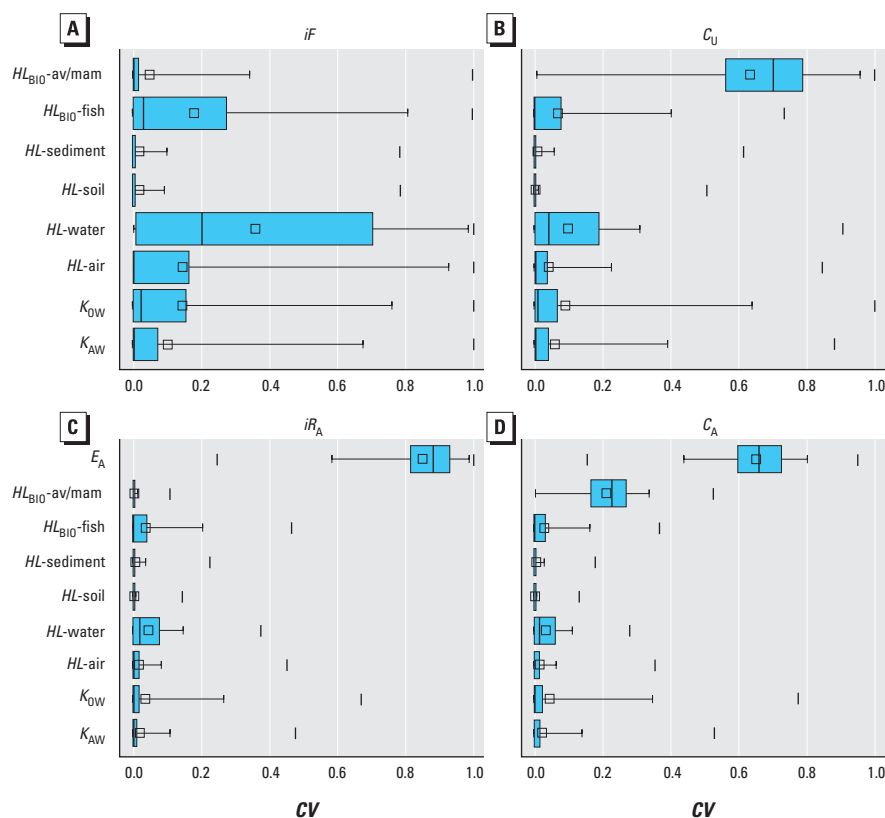
Figure 3. Statistical summary for the CV of model input parameters on the calculated far-field human iF s, C_U s, iR_A s, and C_A s for the 12,619 substances; HL_{Bio-av/mam} , HL_{Bio-avian/mammalian} . Model input parameters are summarized in Table 1. Boxes represent 25th–75th percentiles and whiskers 5th–95th percentiles, vertical lines (|) indicate ranges, lines within boxes are medians, and small squares are means.
